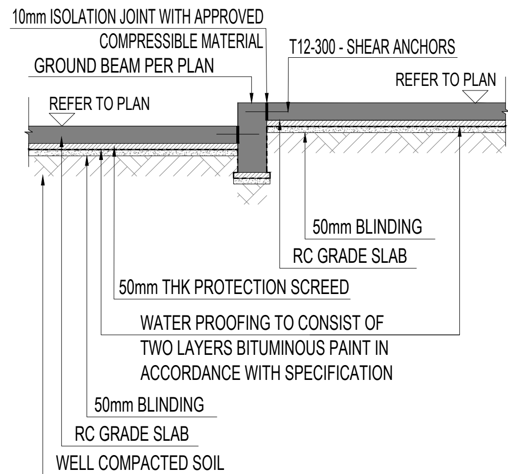
TYP. CONNECTION OF STEPPED SOG TO GB
