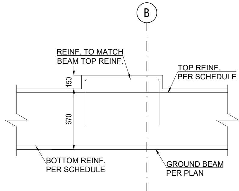
GROUND BEAM BETWEEN STAIRS INFILL
