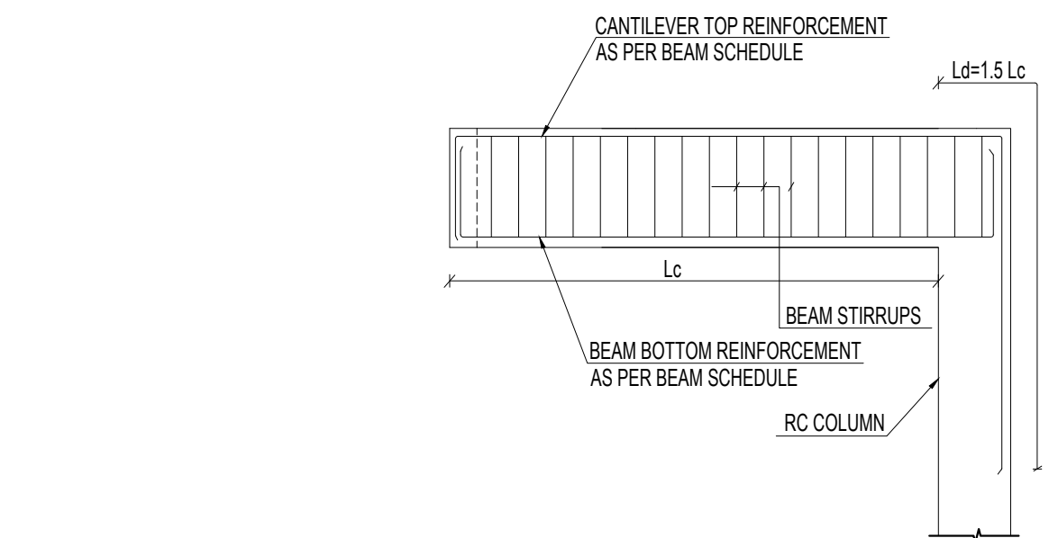
TYP. REINF. DETAIL OF CANTILEVER BEAMS WITH BACKSPAN
