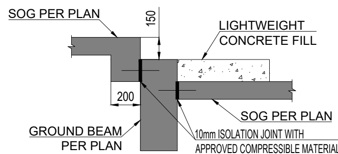
TYP. CONNECTION BETWEEN STEPPED SOG AND GB
