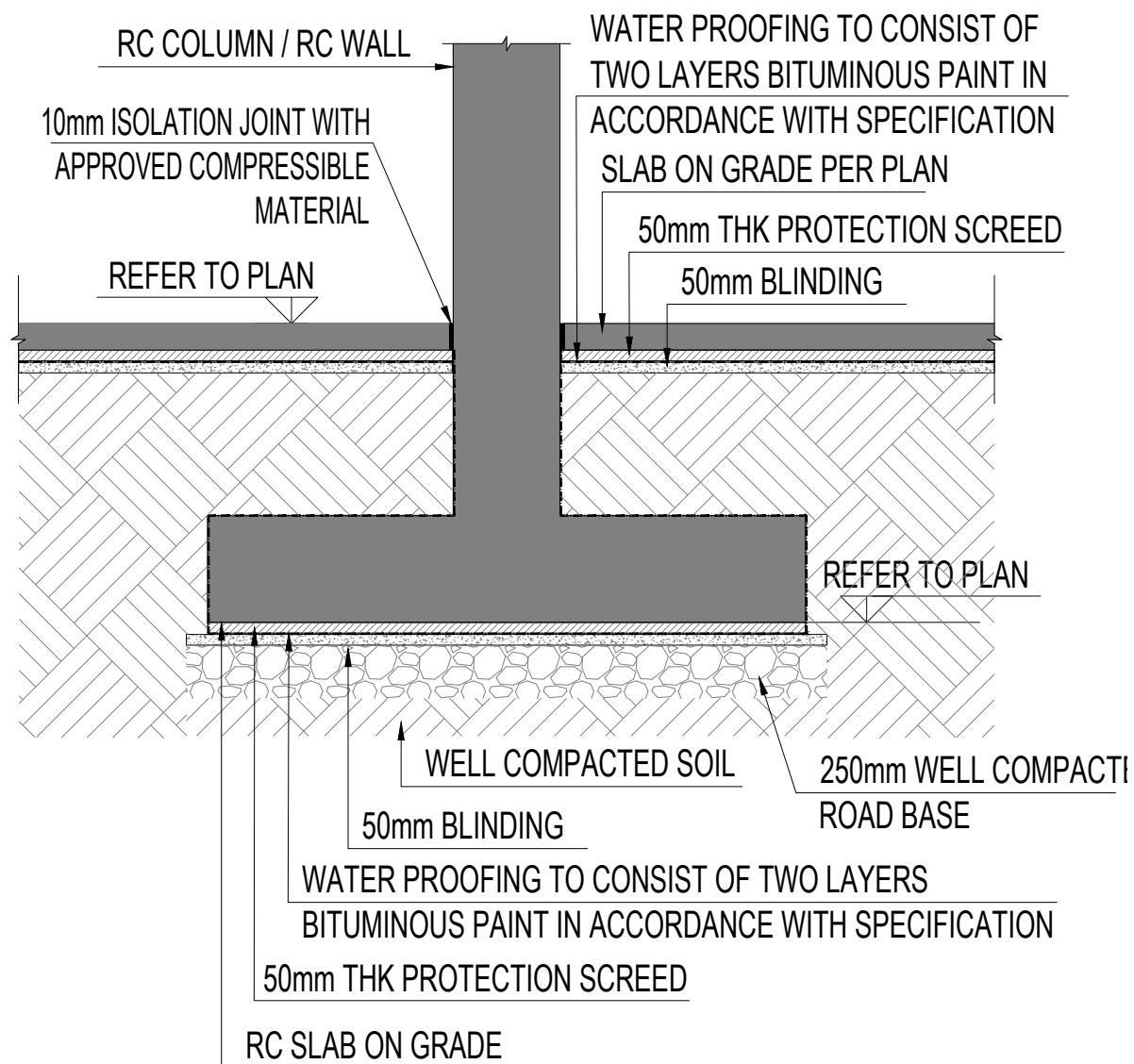
TYP. CONNECTION BETWEEN SOG AND RC COLUMN/WALL
