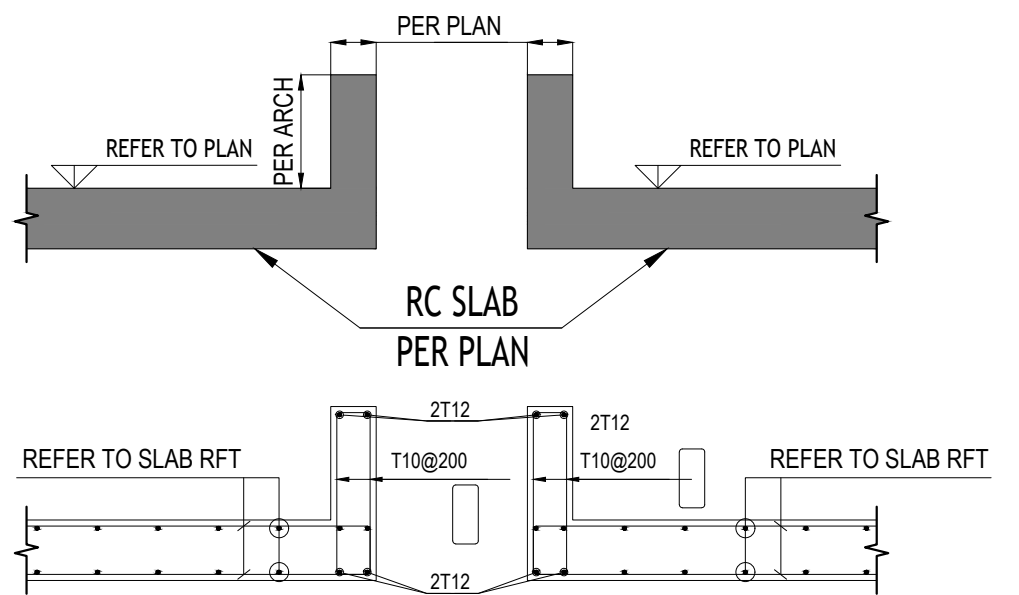
TYP. UPSTAND SECTION
