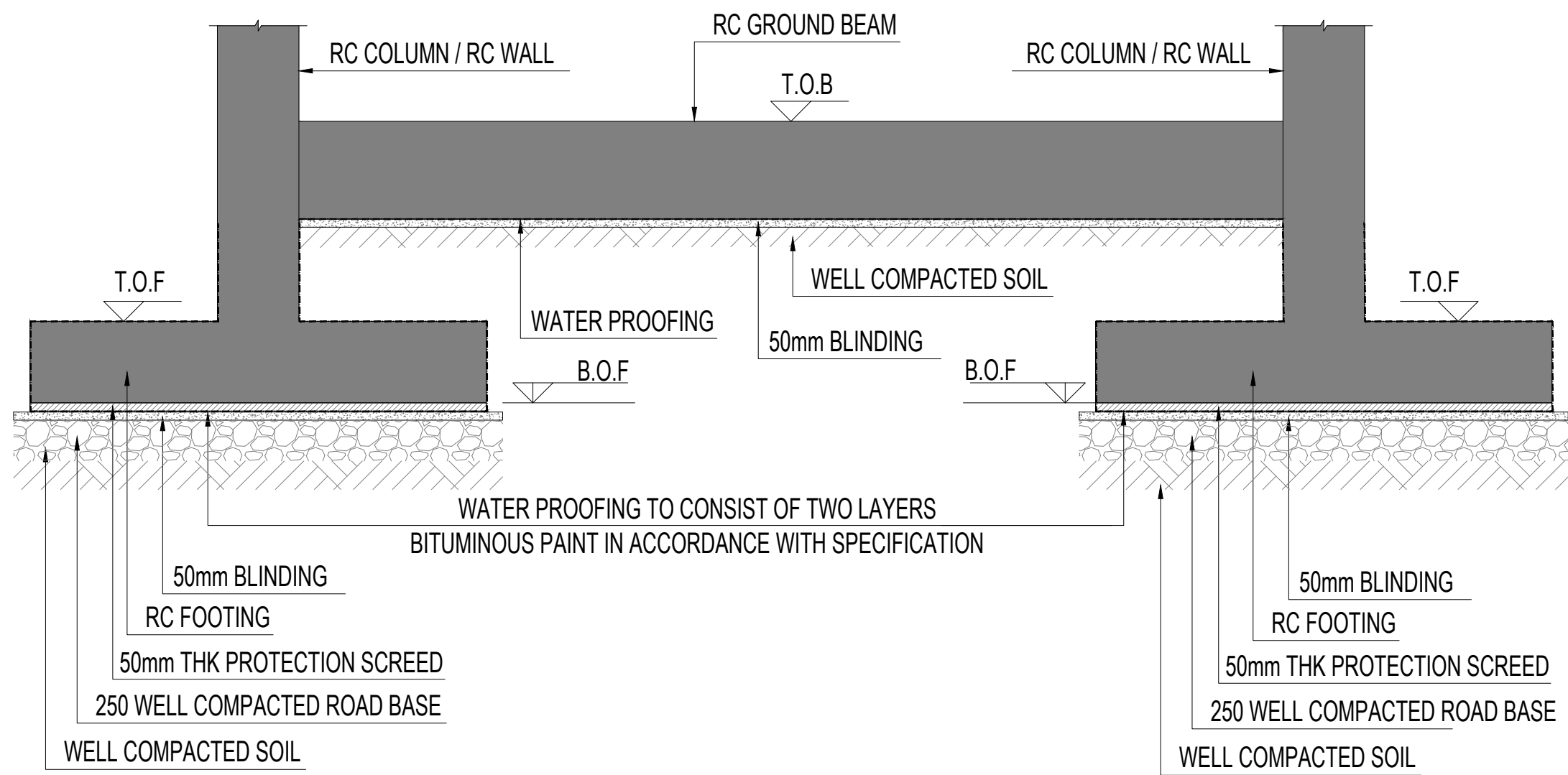
GROUND BEAM TYP. SECTION
