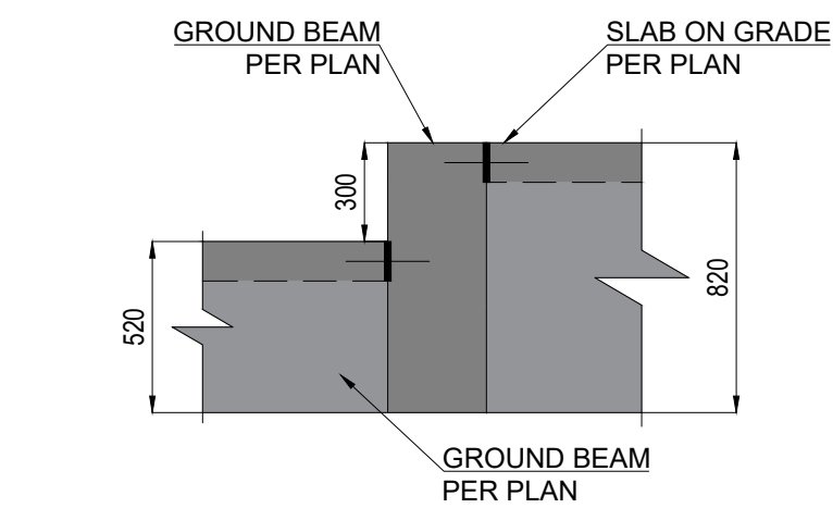
TYP. CONNECTION BETWEEN STEPPED SOG AND GB
